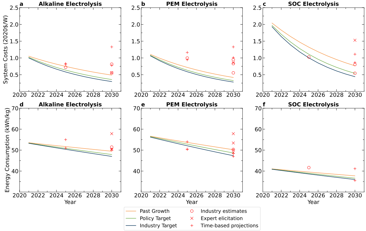
Figure 2. Prospects for system prices and conversion efficiency. a, b, c, d, e, f This figure shows our projections of the potential development of system prices in 2020 $US for (a) alkaline, (b) PEM, and (c) SOC electrolyzers. It also shows our projections of the potential trajectory of energy consumption for (d) alkaline, (e) PEM, and (f) SOC electrolyzers.
