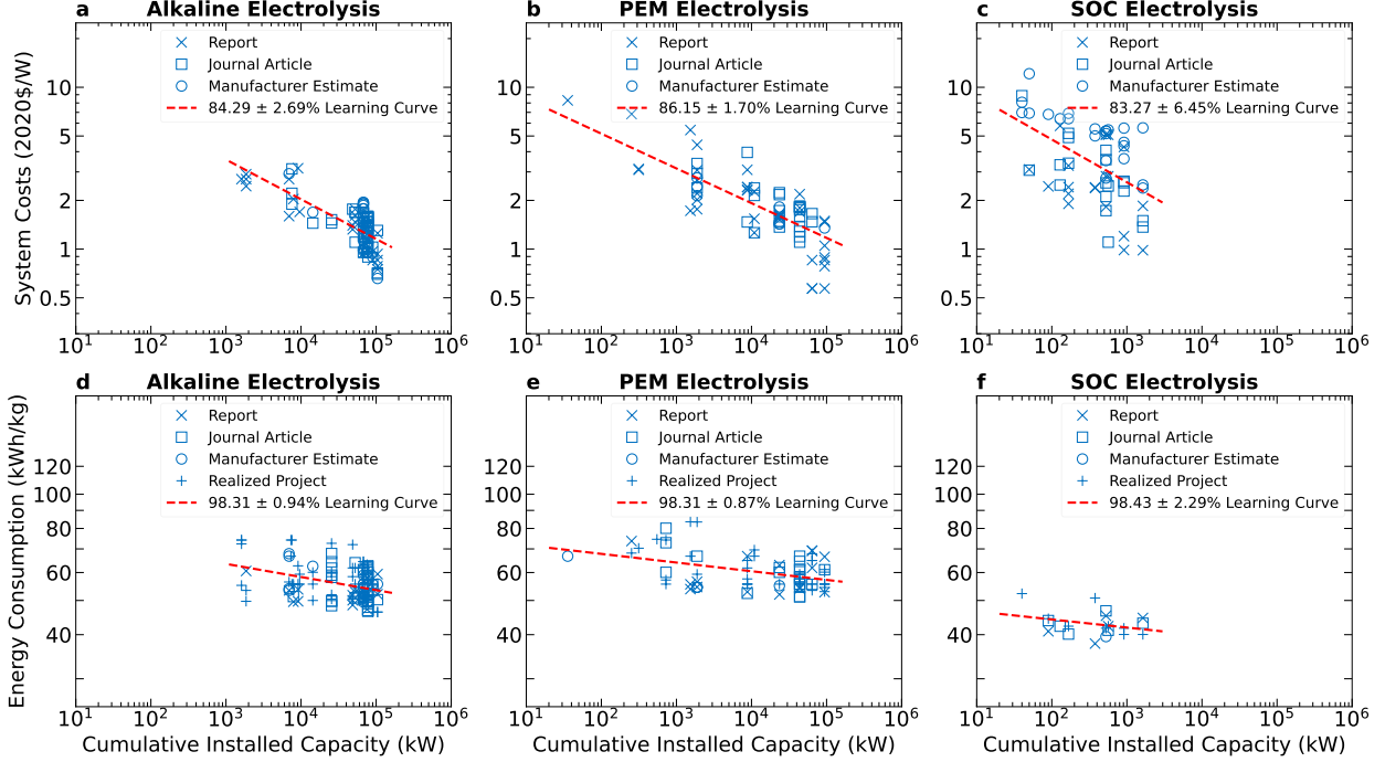
Figure 1. Estimates of learning curves. a, b, c, d, e, f This figure plots the global system prices in 2020 $US against the global cumulative installed capacity together with our estimates of the corresponding learning curves for (a) alkaline, (b) PEM, and (c) SOC electrolyzers. The figure also plots the energy consumption against the global cumulative installed capacity together with our estimates of the corresponding learning curves for (d) alkaline, (e) PEM, and (f) SOC electrolyzers.
