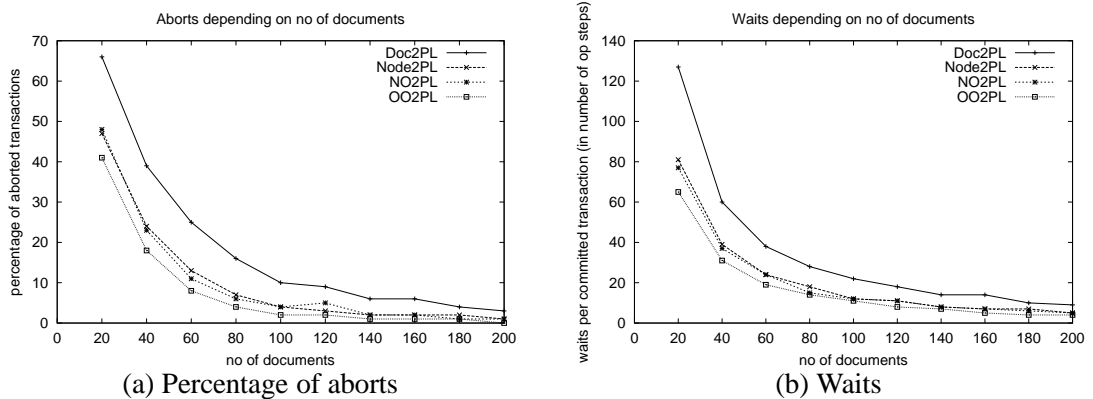
Figure 9: Results varying the number of documents
