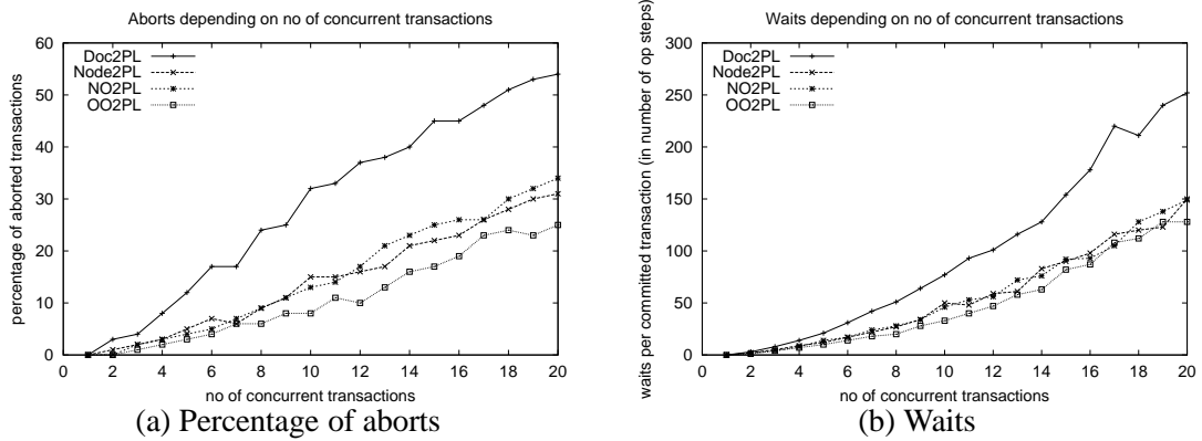
Figure 8: Results for varying the concurrency
